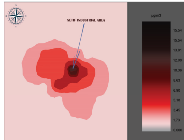
Fig. 11. Daily maximum concentrations of total particles related to the refining operations around the NCEP site (µg/m 3 ).
