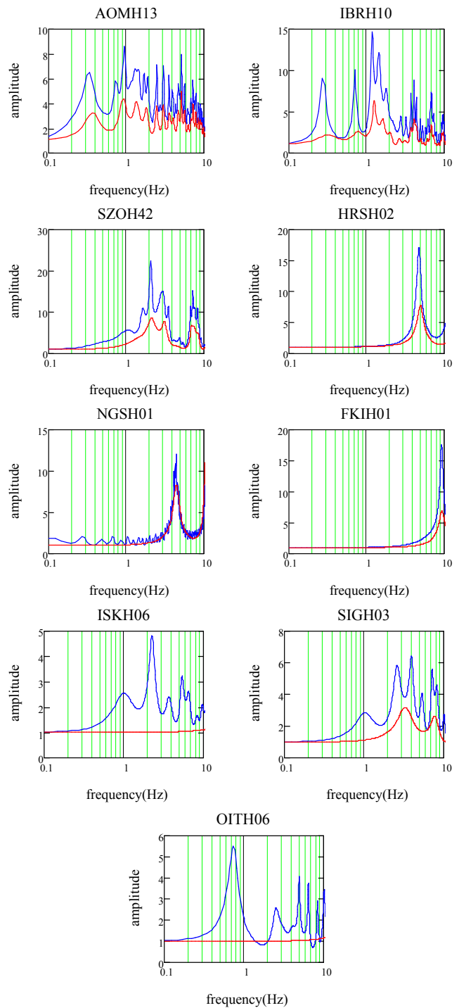
Fig. 3. Transfer function
