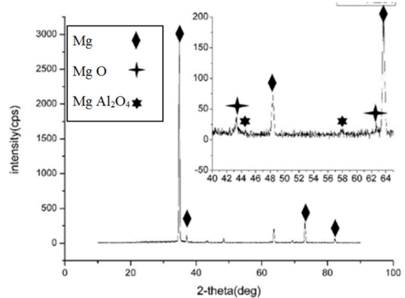
Fig. 3. XRD patterns of MAO coated material rolled at 4.7m/min
