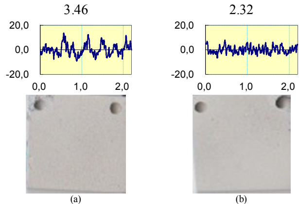
Fig. 4. Surface properties of the examined materials at: (a) 4.7m/min, (b) 10m/min
