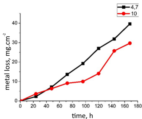
Fig. 5. Corrosion rates of samples that were corroded for 168 hours in 3.5% NaCl
