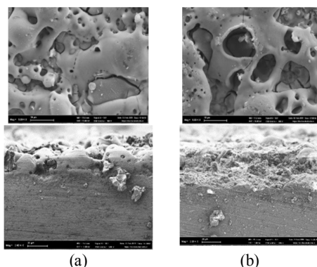
Fig. 2. SEM images of surface and cross-section of materials rolled at: (a) 4.7m/min, (b) 10m/min
