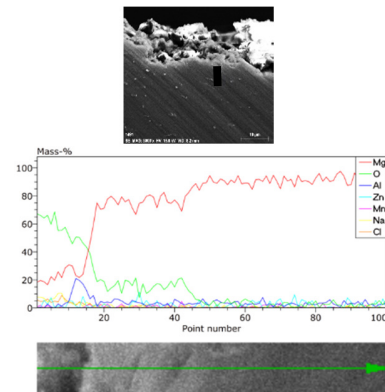
Fig. 7. Linear EDS analysis from section to base material after corrosion test for the 4.7 SP-MAO sample
