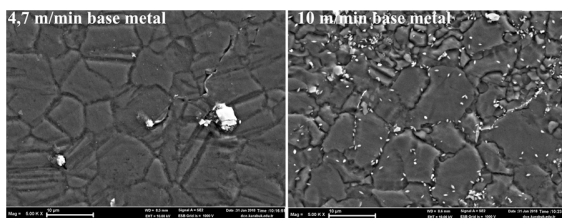
Fig. 1. SEM images of base metals rolled at 4.7 and 10m/min
