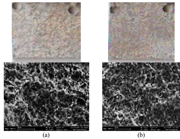
Fig. 6. SEM investigations after the corrosion test, (a) 4.7m/min, (b) 10m/min
