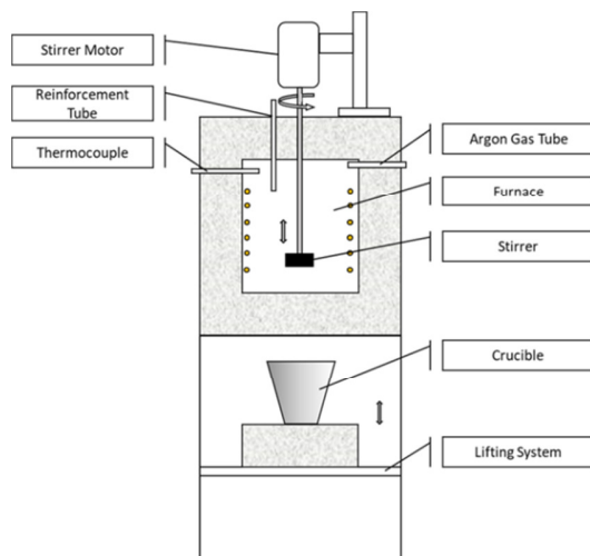
Fig. 1 Mixing casting machine
