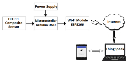
Fig. 4. Hardware block diagram for the environmental monitoring system
