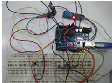
Fig. 6. Hardware Implementation of system design
